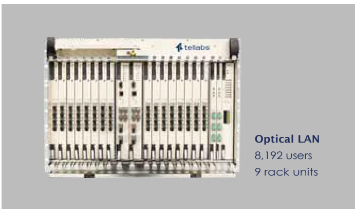
Figure 3. Comparing data center Optical LAN OLT size and density with Active Ethernet LAN
